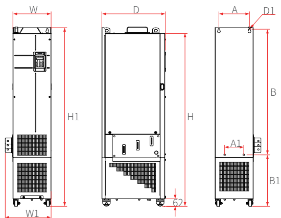
CS710-4T200G-L to CS710-4T400G-L (built-in output reactor)
