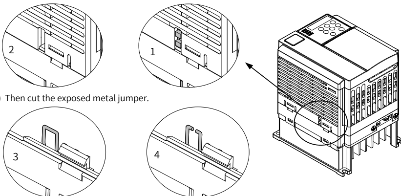
Figure 2-1 EMC jumper position and cutting method of MD310T0.4B to MD310T5.5B
